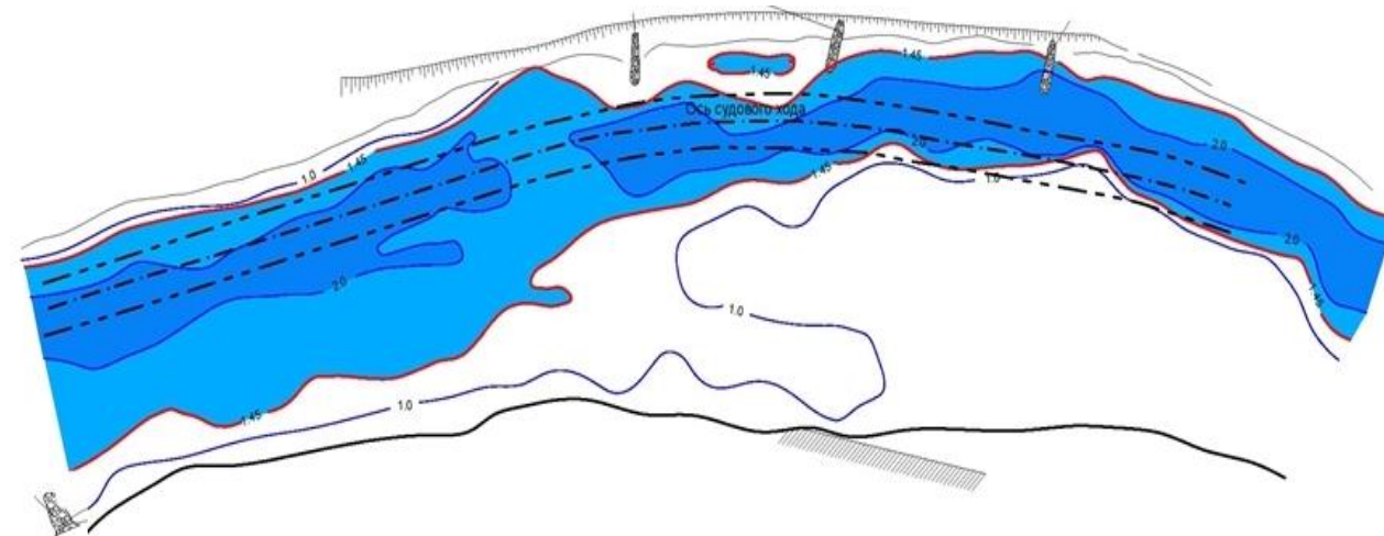
Fairway after Construction the Spur Dikes
