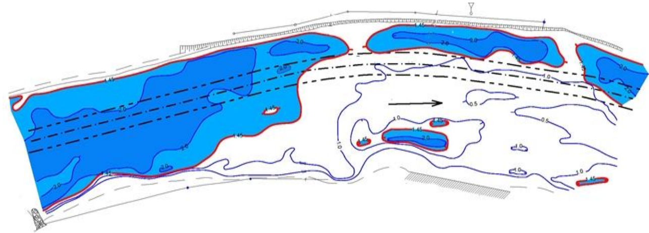
Fairway after Construction the Spur Dikes
