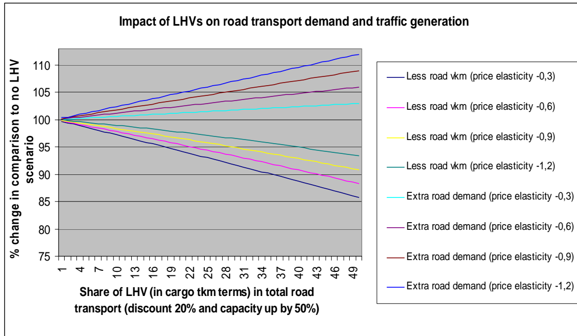
Figure 7: Extra road transport demand and traffic generation
