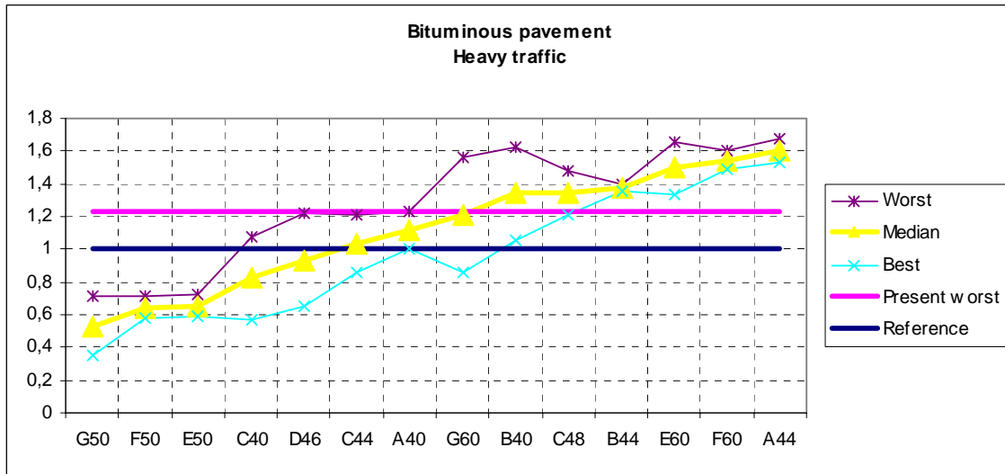
Figure 29: Aggressiveness of each vehicle combination toward bituminous pavements, supporting an heavy traffic
