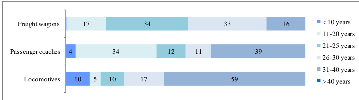
Figure 100: BDZ EAD - Age Structure of Rolling Stock
